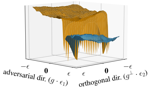
Figure 4: Landscape of the mean value of cosine similarity maps centered around a clean sample x . We calculate the loss value for sample x + \epsilon_1 \cdot \gamma + \epsilon_2 \cdot \gamma^\perp where \gamma is the direction of a successful adversarial attack and \gamma^\perp a random orthogonal direction. The different colors indicate the predicted class of the neural network, with orange indicating the correct class.
