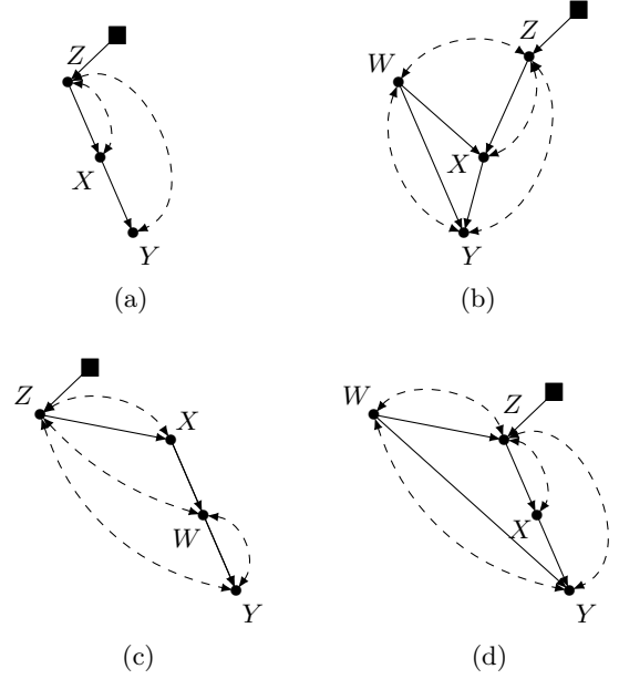
Figure 2: Selection diagrams where P_x(y) is zTR , but not ID , with an experiment on Z . A selection variable S is represented by a black square \blacksquare .
