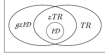
Figure 3: A Venn diagram depicting Theorem 3. Given a selection diagram D and controllable variables \mathbf{Z} , the intersection of gzID and TR relations exactly matches to zTR relations in any model that induces D .
