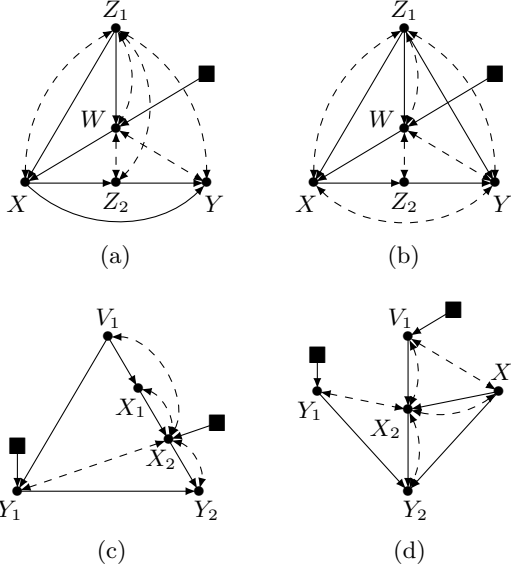
Figure 5: Selection diagrams where P_{\mathbf{x}}(\mathbf{y}) is not \mathcal{ID} but zTR but given controllable variables \mathbf{Z} ( V_1 and X_2 are controllable variables for Figure 5(c) and 5(d)).
