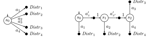
(a) Four actions in a POMDP
